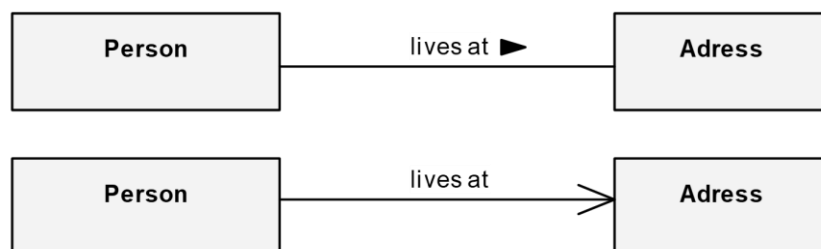
Figure 27: Reading direction vs. navigability
