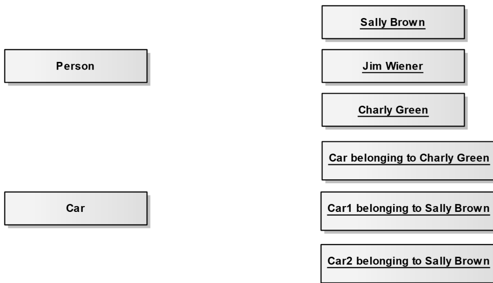
Figure 10: Class vs. object
