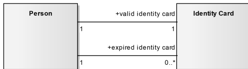
Figure 29: Resolution of unknown multiplicities
