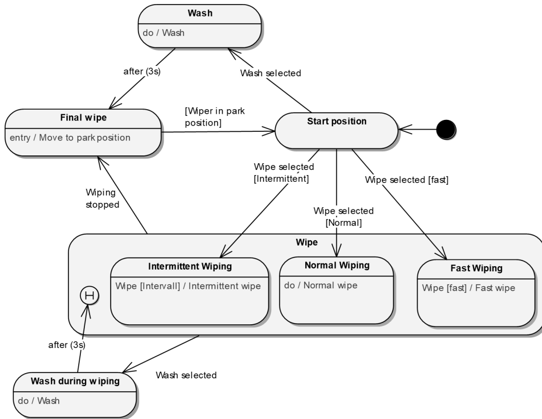
Figure 54: State diagram for a wiper system
