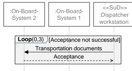
Figure 87: Modeling of a combined fragment of the type "loop"
