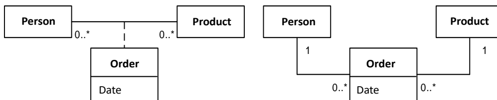
Figure 14: Transformation of modeling of association classes by using “normal“ classes
