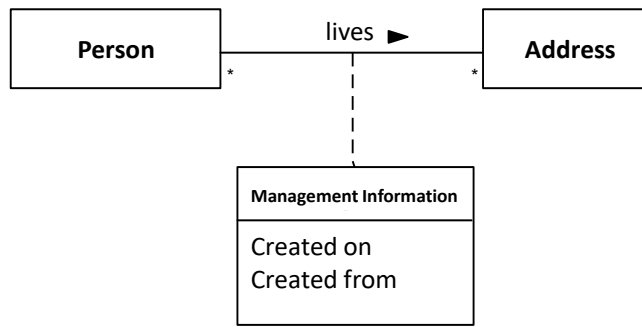
Figure 23: Simple Example of modeling management information with association classes
