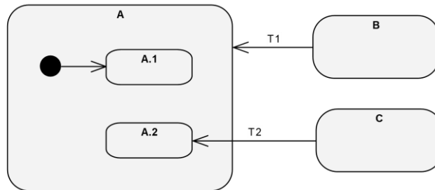
Figure 64: Entry into composite states
